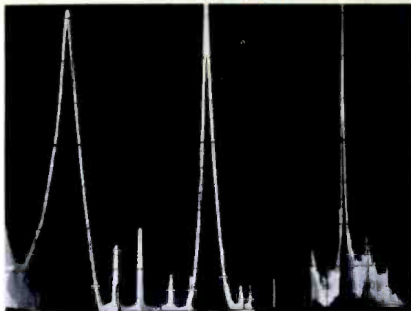
Figure 1. Shown here are 70, 700, and 7000Hz test tones and harmonics at tape deck output. Harmonics for 70Hz are -50dB or 0.3 percent. For 700Hz, -60dB or 0.1 percent, and -50dB for 7000Hz or 0.3 percent.
